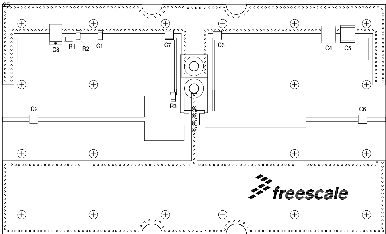
Figure 3. MMRF1014NT1 Test Circuit Component Layout
