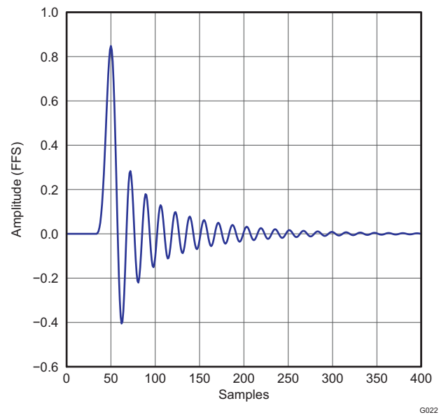
Figure 27. Low latency x8 Interpolation Filter Impulse Response
