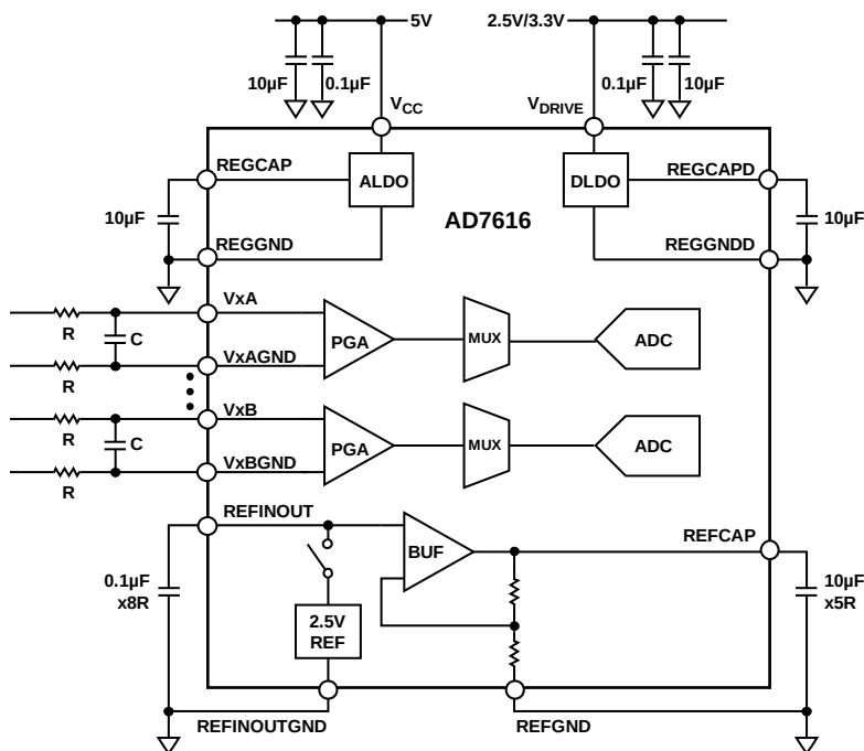
Figure 49. Typical External Connections
