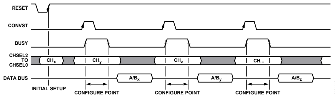
Figure 51. Hardware Mode Channel Conversion Setting
