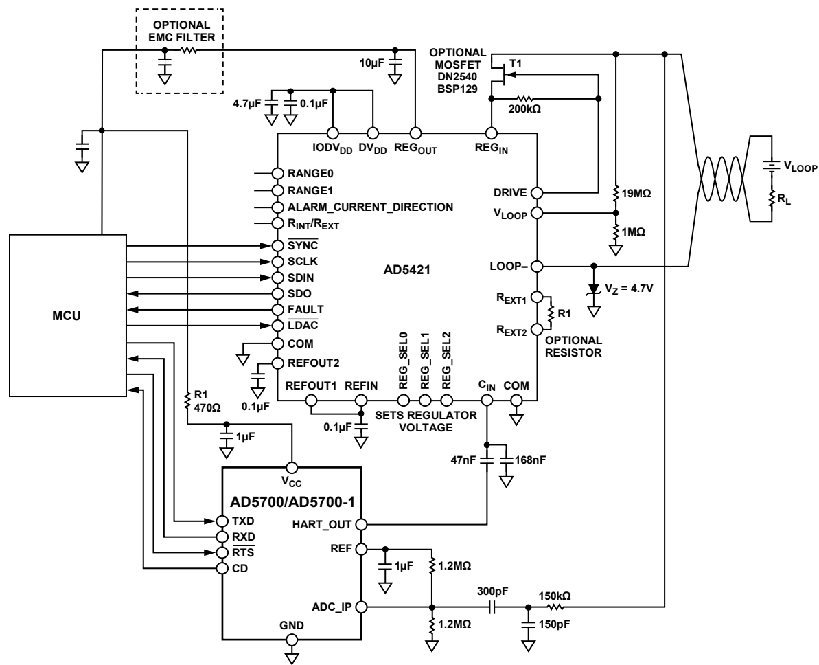
Figure 27. Loop-Powered Transmitter Diagram
